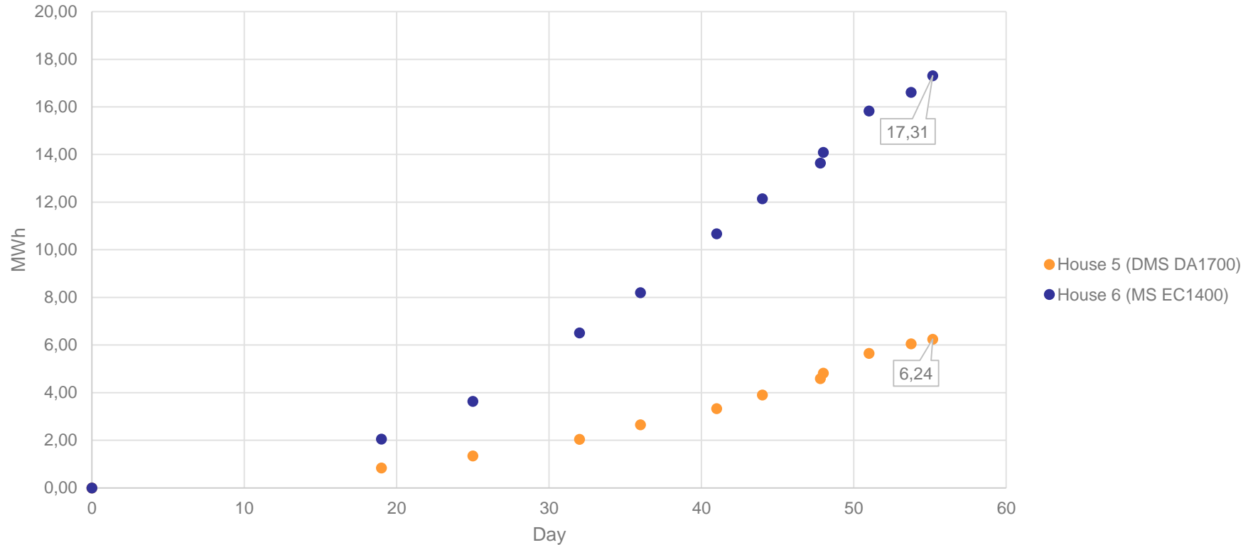
CT Ventilation Powerconsumption Batch start 05-11-2016
