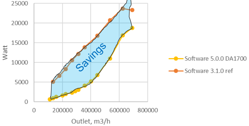
Tunnel mode
