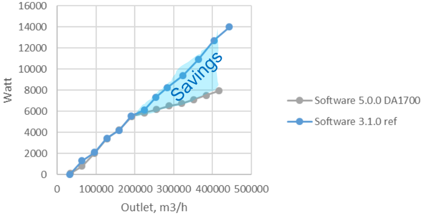
Side mode
