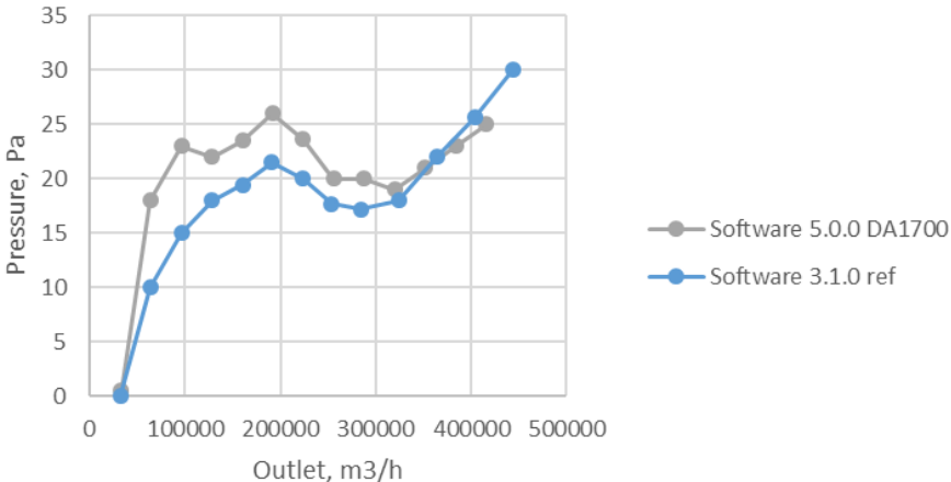
Side mode
