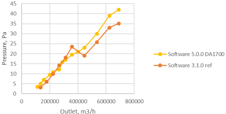
Tunnel mode
